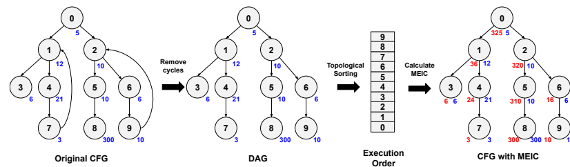
Figure 4. Overview process of calculating Maximum Expectation of Instruction Count (MEIC). The blue number (number at the right side of each node) shows the instruction count of the basic block and the red number (number at the left side of each node) shows MEIC of the basic block.
